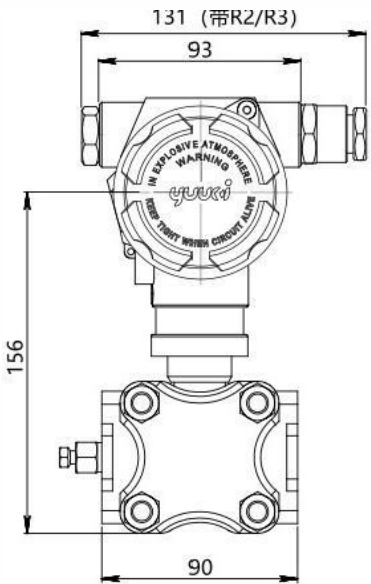
Size drawing of the whole machine without display function
