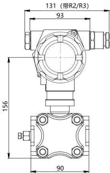
Overall size drawing with display function
